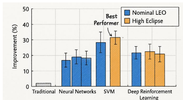
Figure 4. Improvement in energy efficiency ( R_{energy} ) for Nominal LEO and High Eclipse scenarios using traditional neural networks, SVM, and deep reinforcement learning. Synthesized from Yaqoob et al. (2022), Baccari et al. (2025), Ortiz et al. (2023), and Shakoor (2025).
