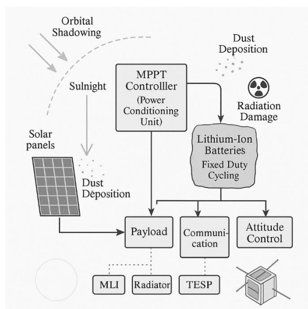
Figure 2. Schematic diagram of a traditional Electrical Power System (EPS) in a CubeSat, illustrating energy flow from solar panels through an MPPT controller and lithium-ion batteries (with fixed duty cycling) to subsystems (payload,
