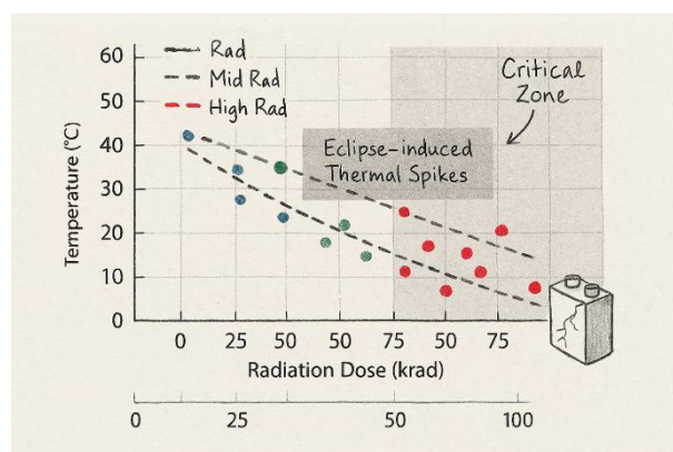
Figure 1. Relationship between radiation dose (kRad) and temperature (°C) in CubeSat batteries, highlighting eclipse-induced thermal spikes and the critical zone. Adapted from Rahman (2023) and Pathak et al. (2023).
